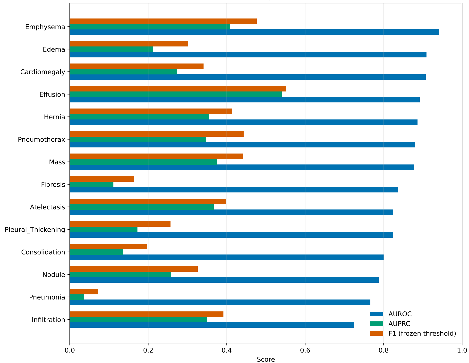
Per-class test performance
