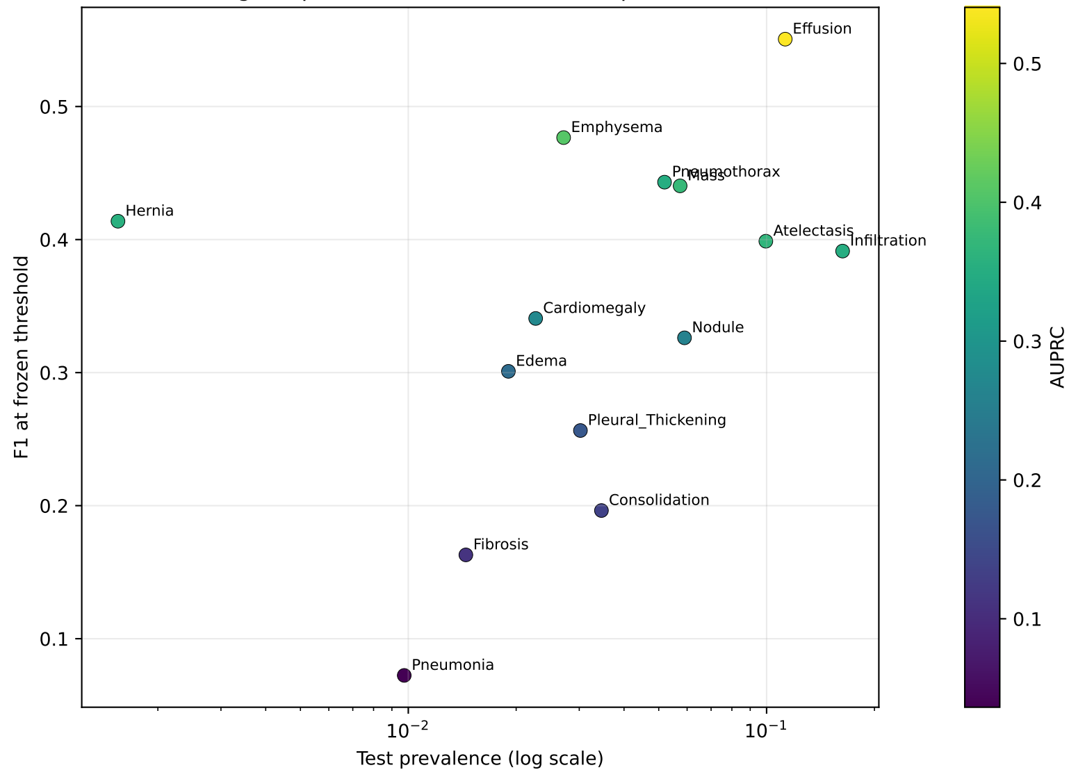
Long-tail prevalence and thresholded performance
