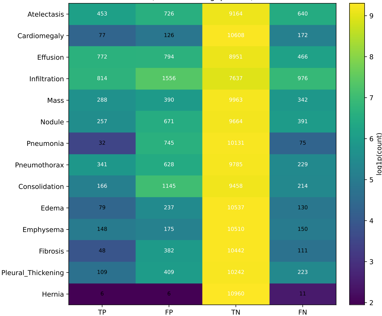
Test confusion counts at frozen validation thresholds (color scale: log1p count)
