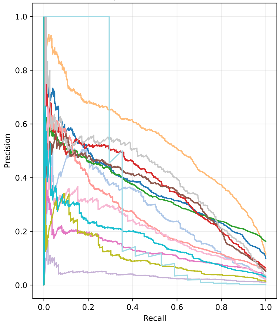
Test precision-recall curves
