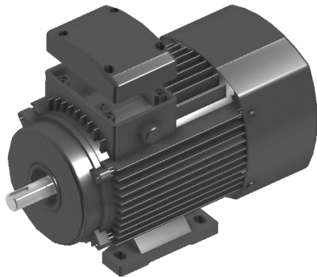
Integrated Junction Box (Aluminum Case)
