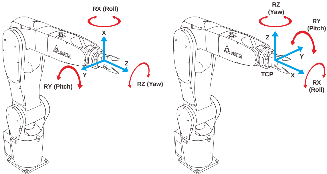
Tool Frame directions by default and after rotation
