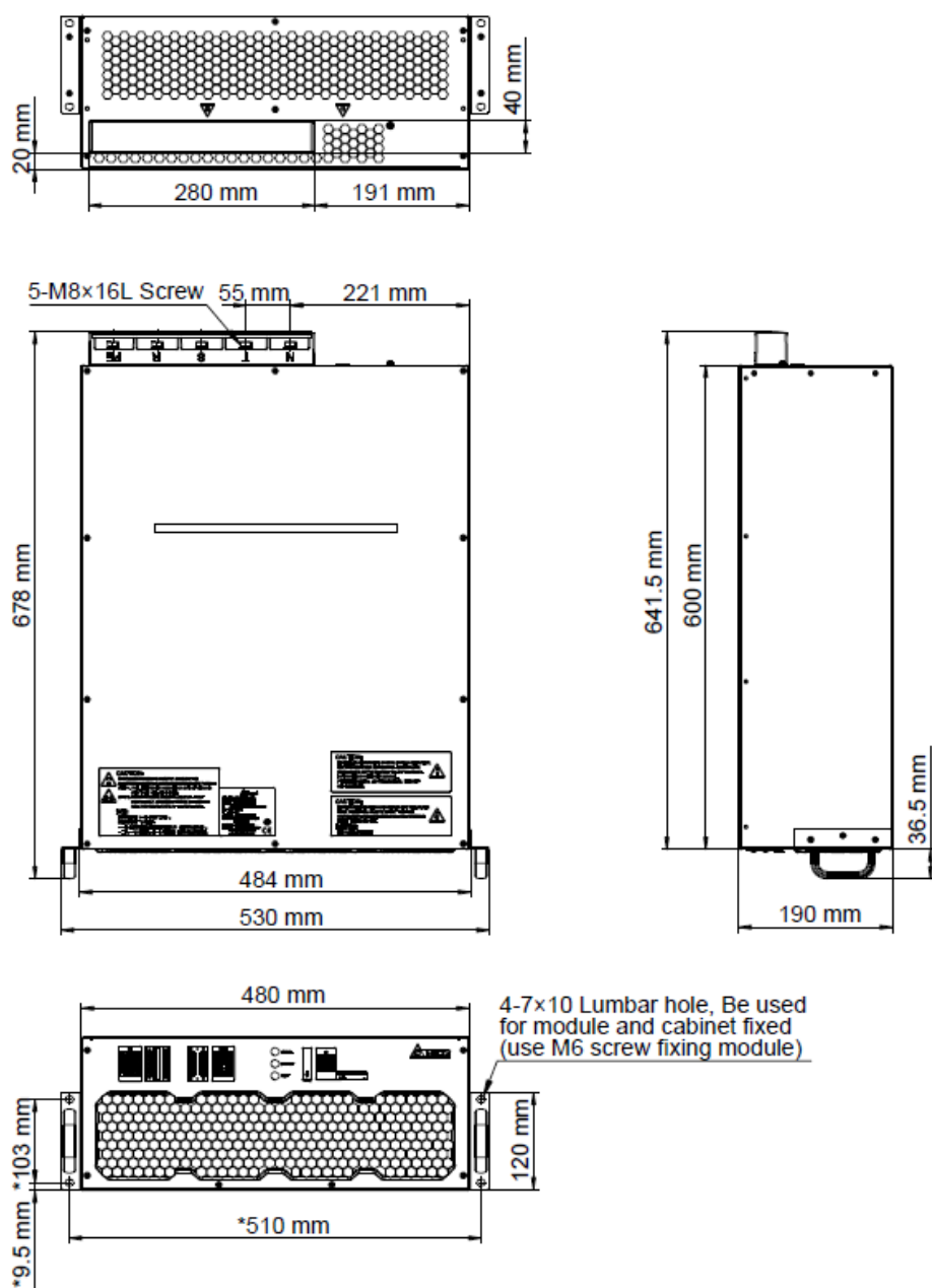
(Figure 3-9: APF Module Dimensions_ 30 A/ 50A/ 70A Models)
