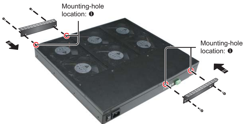
(Figure 3-c) Mount the Bracket Ears
