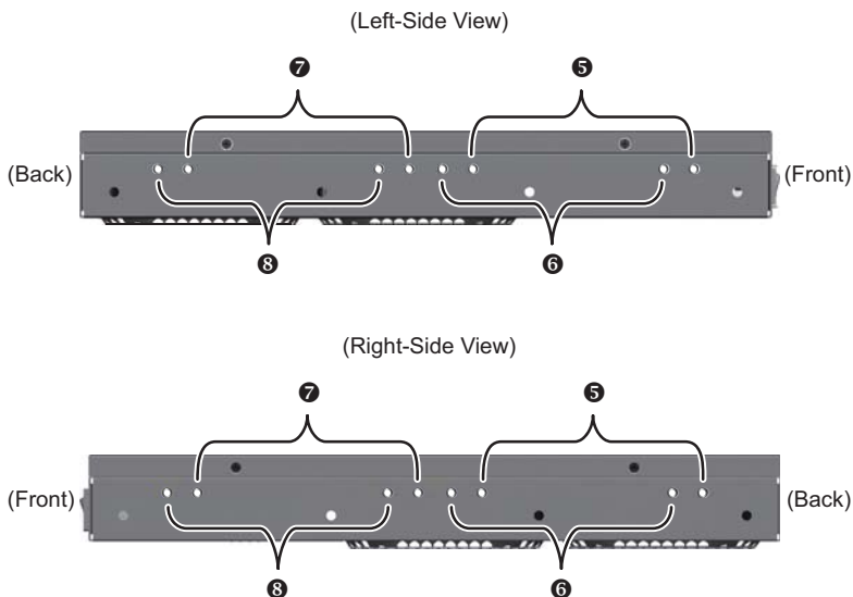
(Figure 3-b) ADU's Mounting-hole Locations (Left and Right)
