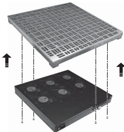
(Figure 3-d) Mount the ADU under a Raised Floor
