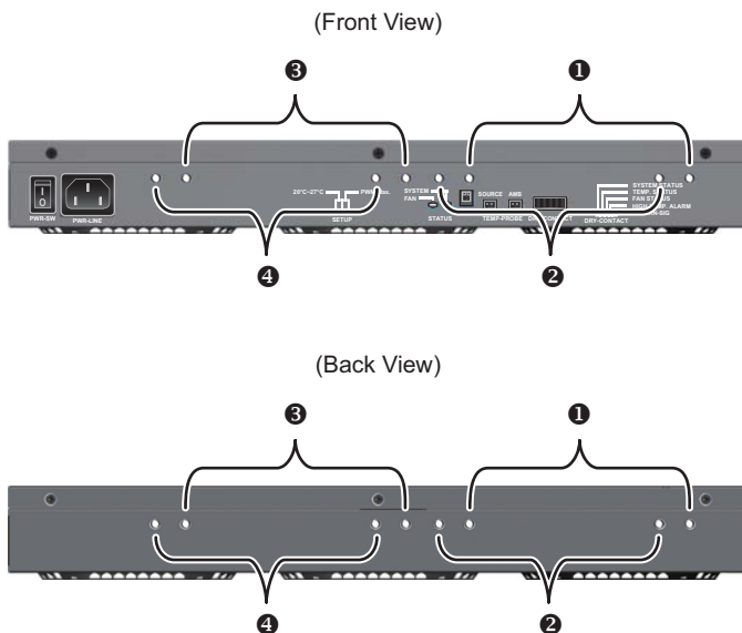
(Figure 3-a) ADU's Mounting-hole Locations (Front and Back)
