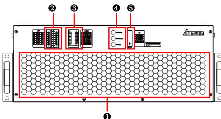
(Figure 2-8: 50kvar&100kvar SVG_ Front of the Module)
