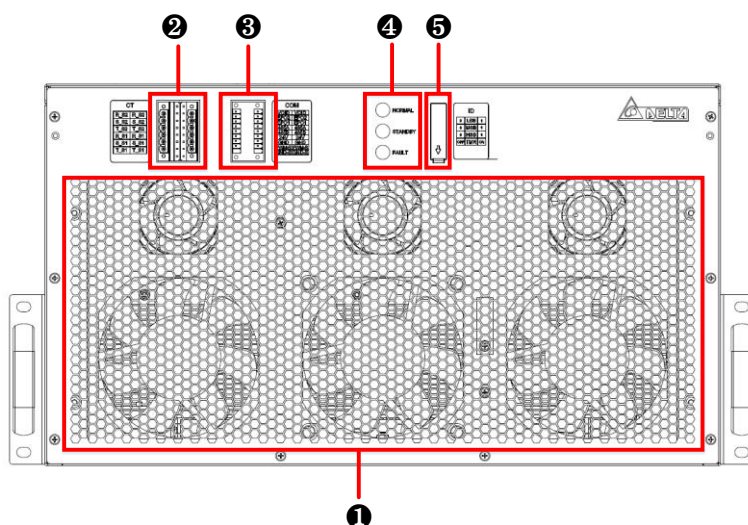
(Figure 2-10: 150kvar SVG_ Front of the Module)
