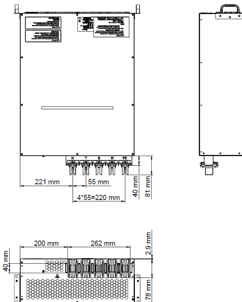
(Figure 3-14: SVG Module Dimensions_ 50kvar Modules (After Combination with Pluggable terminals))
