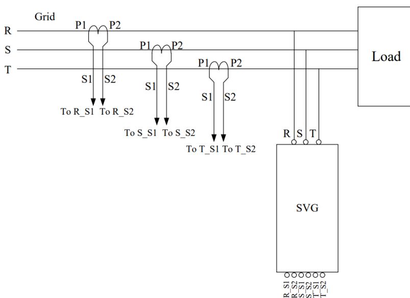
(Figure 3-28: Basic CT Installation and Wiring Diagram_ Close Loop)
