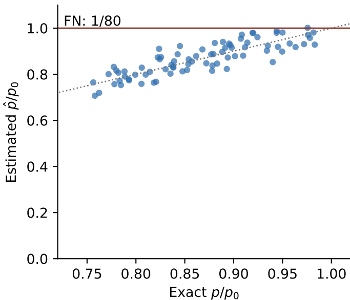
HEP-like — Smooth MCMC-IS
