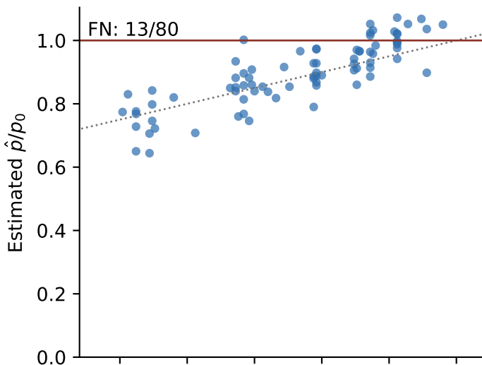
GWAS-like — Smooth MCMC-IS
