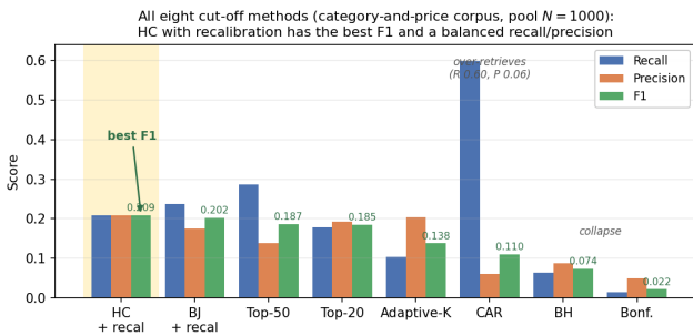
Figure 2: All eight cut-off methods on the category-and-price corpus (pool N=1000 ). HC with recalibration (highlighted) has the best F1 and a balanced recall/precision; the cluster rule (CAR) over-retrieves to a high recall but near-zero precision, and the family-wise-error (Bonferroni) and false-discovery (BH) rules collapse to almost nothing.
