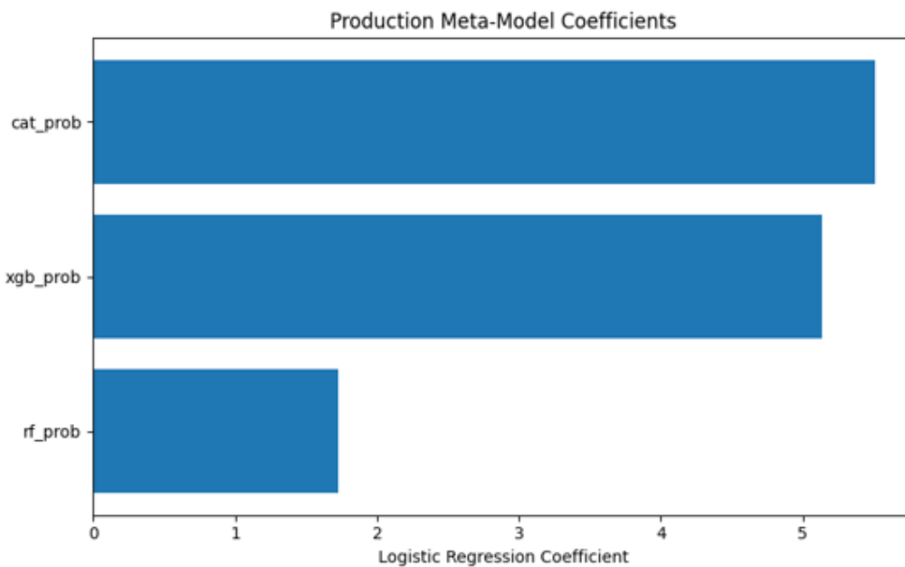
Figure 31: Logistic Regression coefficients learned for the three probability meta-features of the selected Random Forest–CatBoost–XGBoost ensemble.
