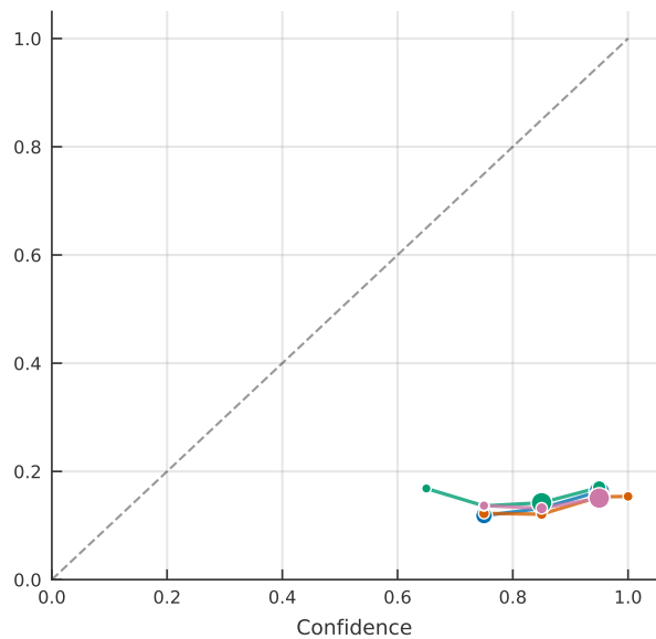
MedEval
