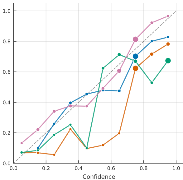
LifeEval
