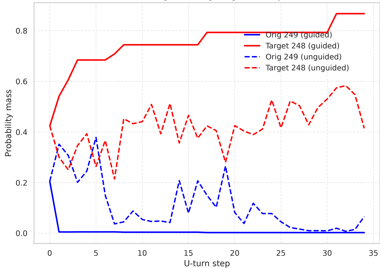
Guided vs Unguided: Dog→Dog Probability Mass
