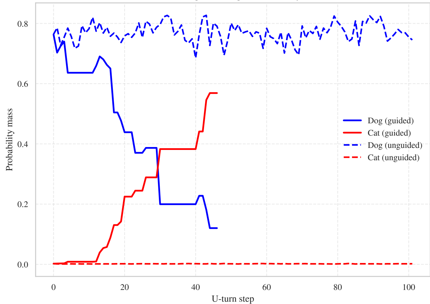
Guided vs Unguided: Dog/Cat Probability Mass
