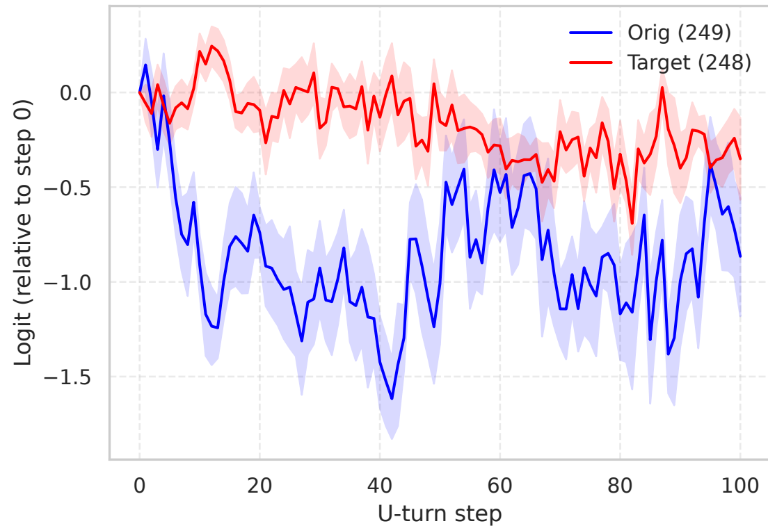
Unguided (dog→dog): Potential
