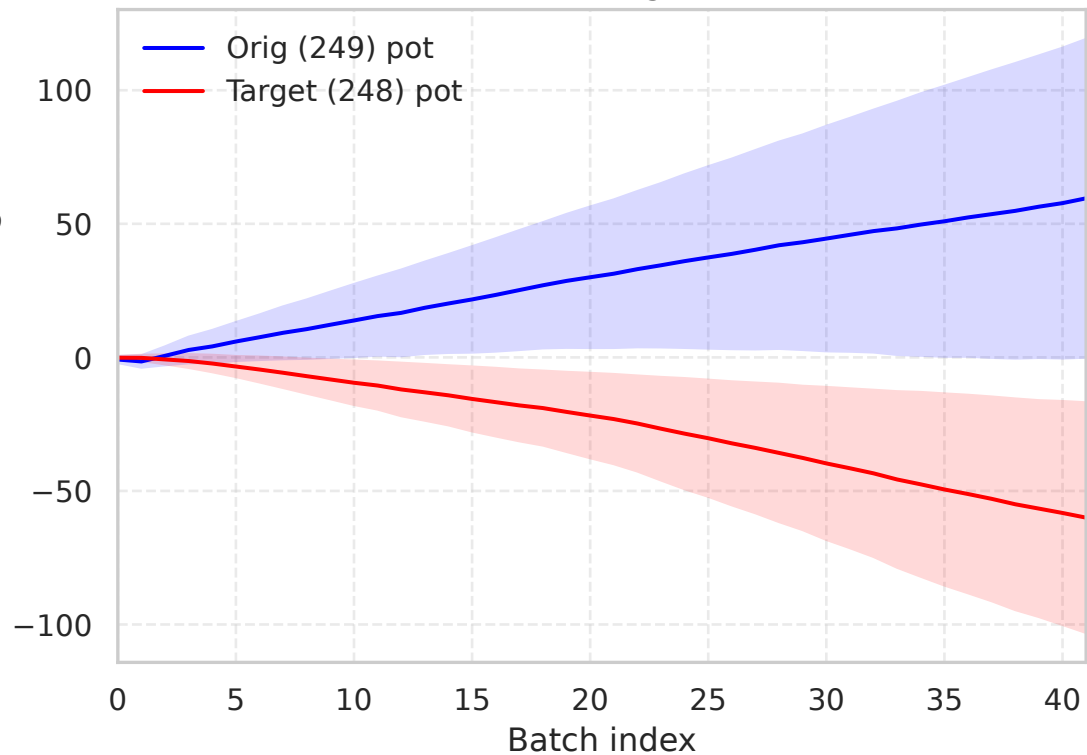
Guided (batch-avg): Potential
