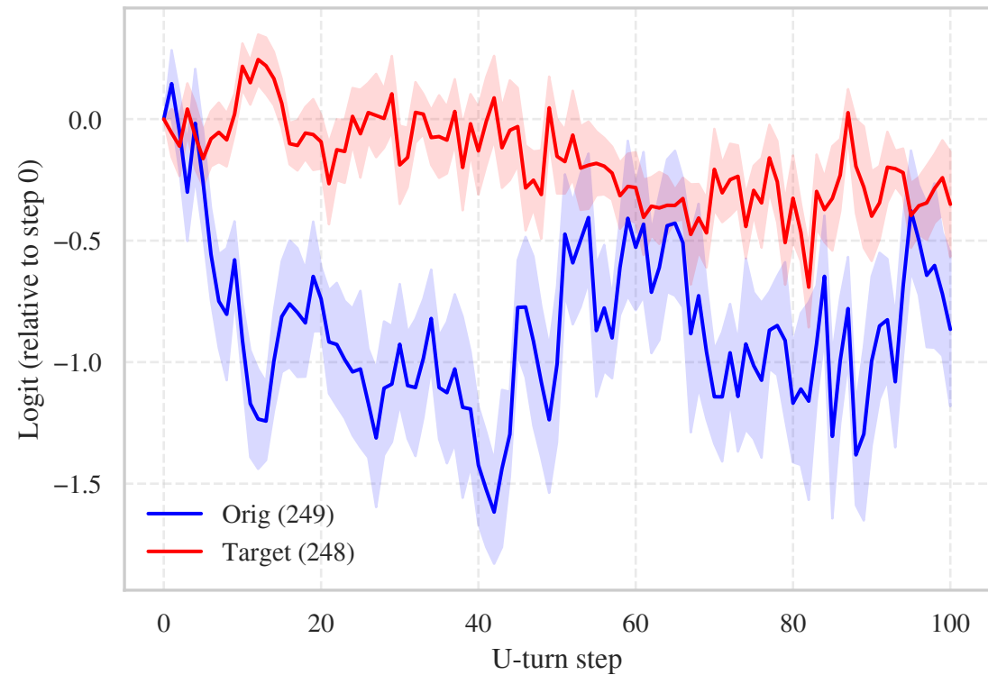
Unguided (dog→dog): Potential
