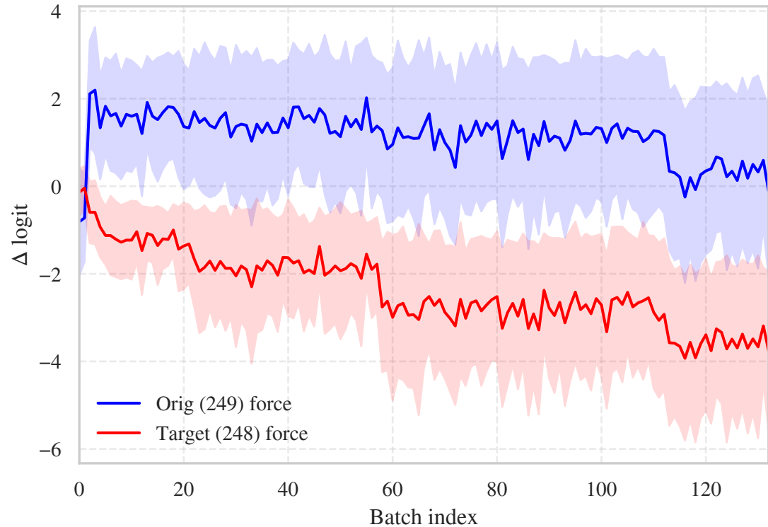
Guided (batch-avg): Force ( \Delta \text{logit} )
