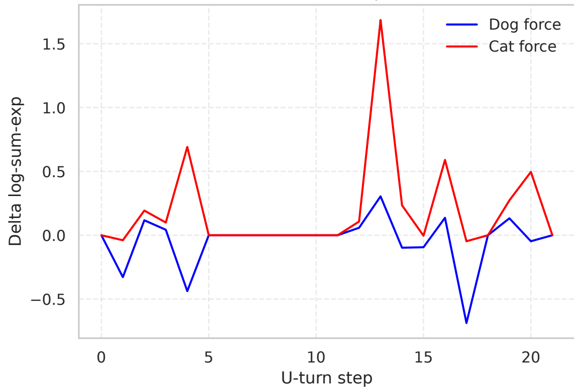
Guided: Force (Delta potential)
