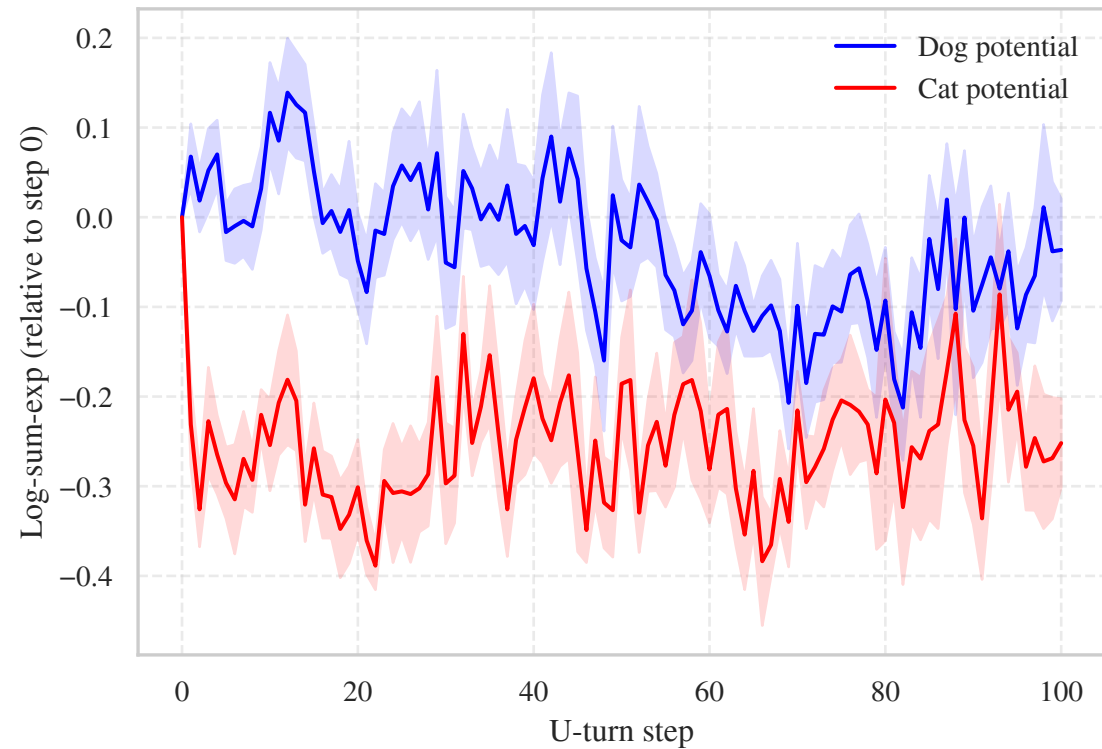
Unguided: Potential
