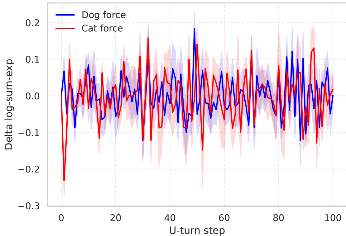
Unguided: Force (Delta potential)
