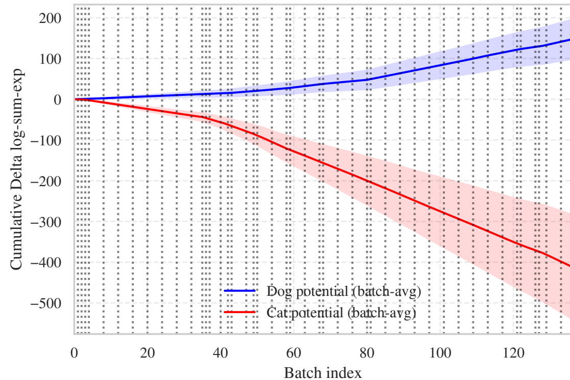
Guided (batch-avg): Potential
