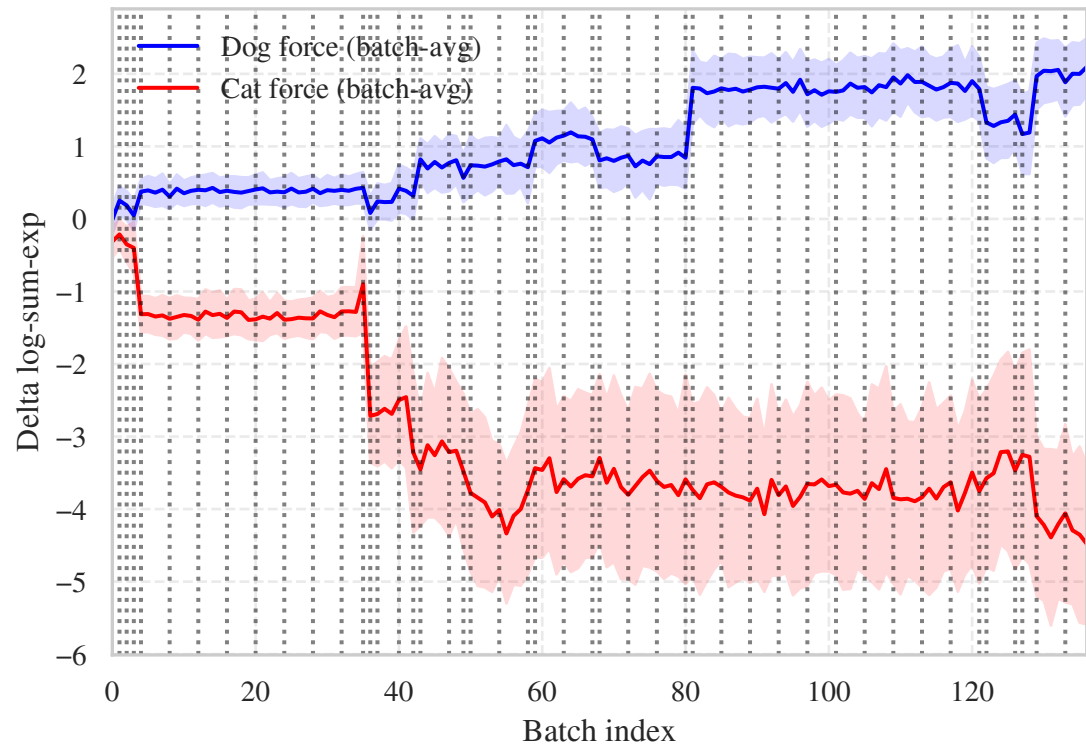
Guided (batch-avg): Force (Delta potential)
