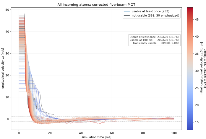
Five-beam: a useful subset is captured, while many trajectories leave after slowing or reversal.
