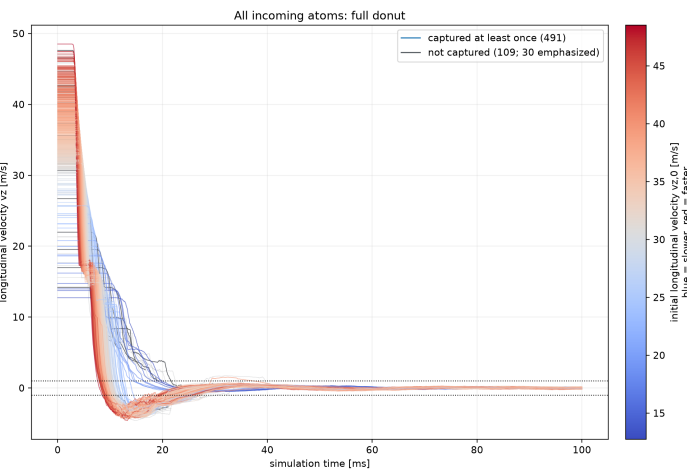
Donut: broad entrance-velocity acceptance and stable slowing into the usable band.
