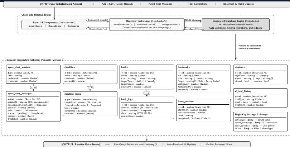
Figure 4.4: Browser IndexedDB Database Schema and Reactive Data Architecture (PrismDB)
