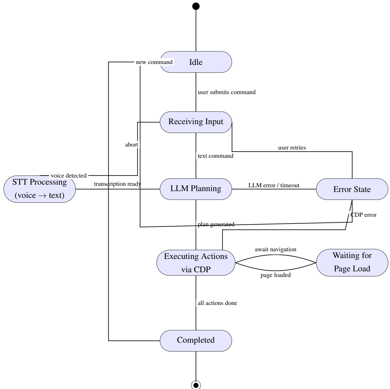
Figure 6.4: State Chart Diagram – AI Agent Command Lifecycle
