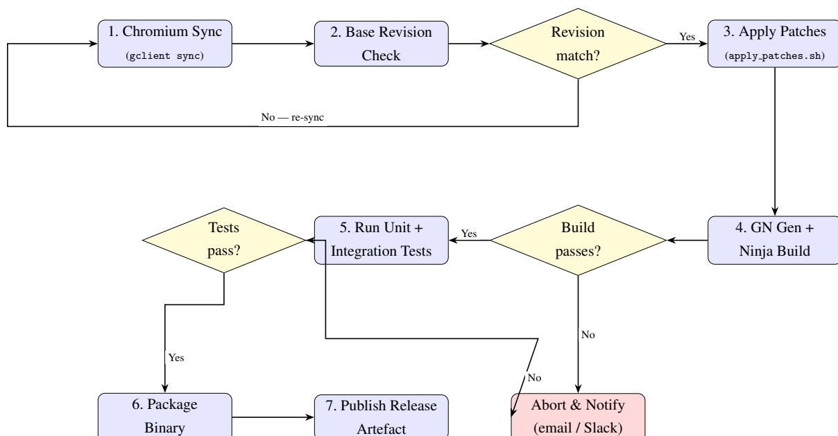
Figure 7.1: CI/CD Pipeline – Prism AI Browser
