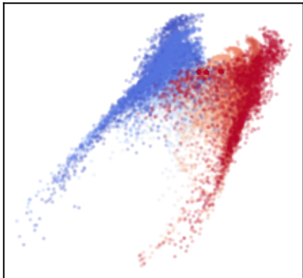
contrastive s2
