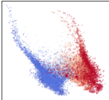
contrastive s4
