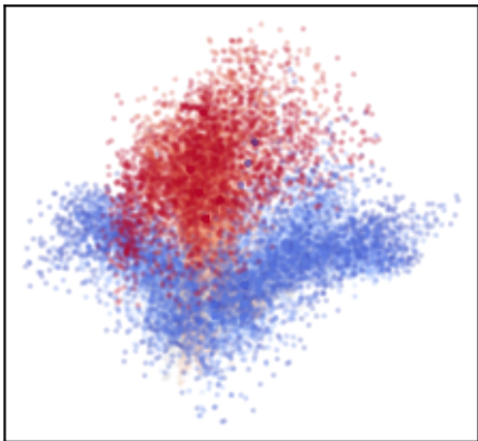
contrastive s1
