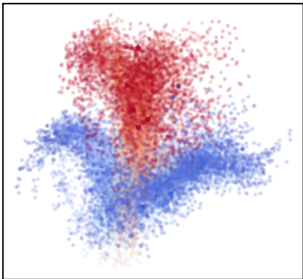
contrastive s0
