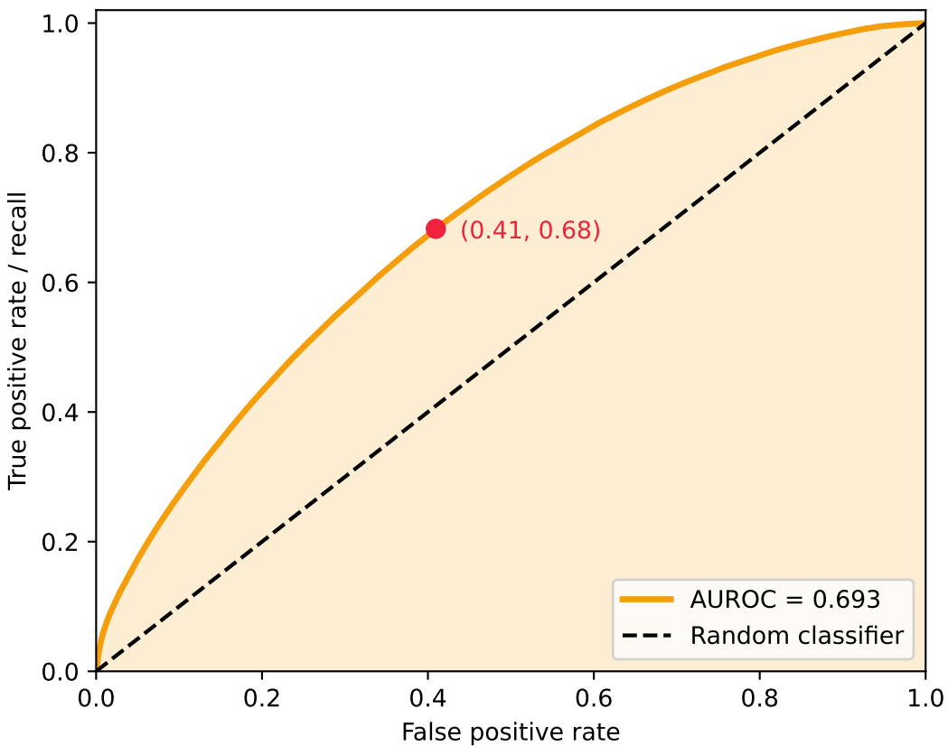
chr16: ROC curve
