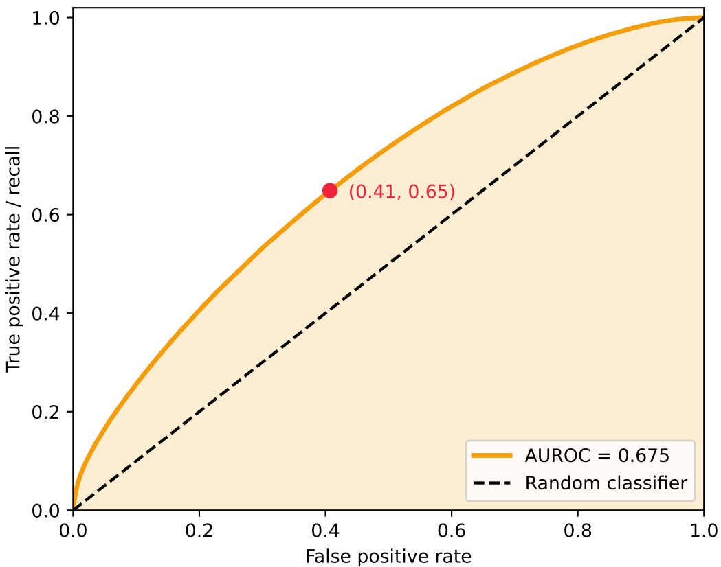
chr17: ROC curve
