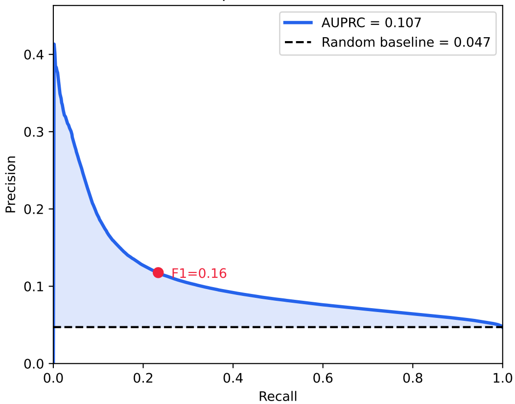
chr17: precision-recall curve
