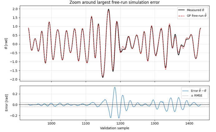
Fig. 1: Zoomed free-run simulation of the best GP-NARX model with n_a = 5 and n_b = 5 . The upper plot compares the measured disk angle with the recursively simulated GP trajectory. The lower plot shows the signed simulation error \hat{\theta} - \theta , together with the \pm RMSE reference lines.
