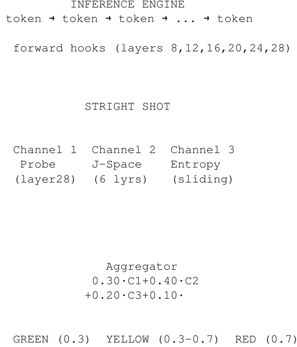
Figure 1: StrAIght Shot system architecture. Forward hooks at six strategic layers capture hidden states and route them to three parallel detection channels. The weighted aggregator emits a GREEN/YELLOW/RED verdict per token.
