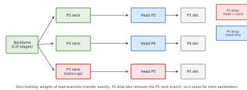
Figure 1: What is dropped. P3-drop removes only the P3 branch of the detect head; P5-drop additionally removes the P5 neck branch (conv + upsampling), which is why it saves far more parameters and FLOPs.
