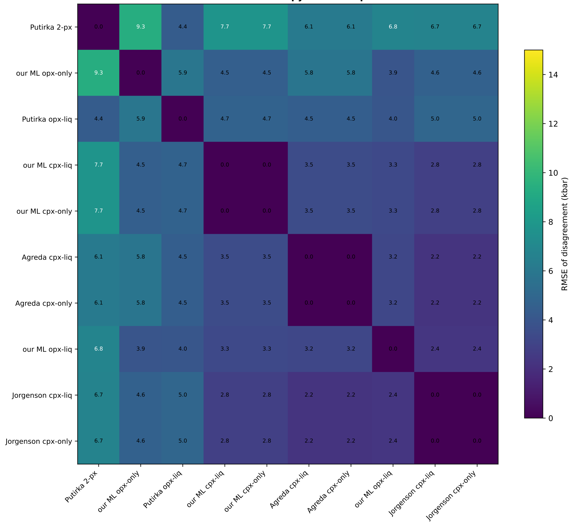
Method Agreement Matrix - P (kbar) LEPR natural two-pyroxene corpus
