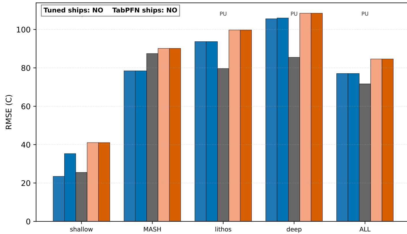
(c) Opx only T (C)
