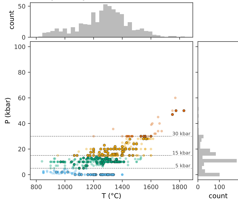
(a) Opx + Liquid
