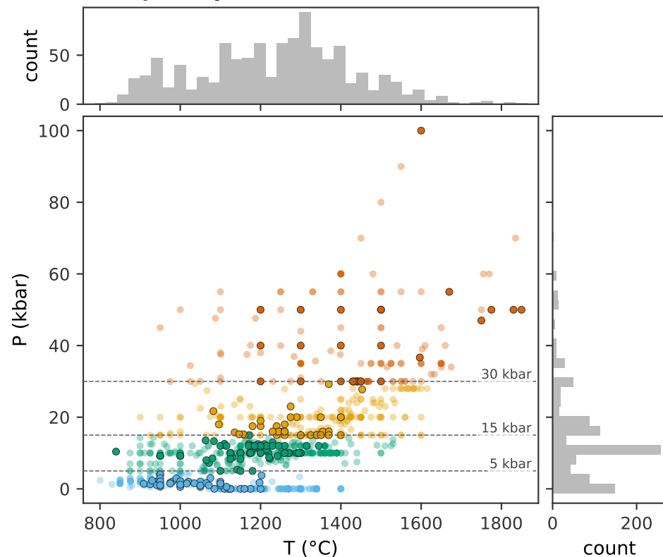
(b) Opx only
