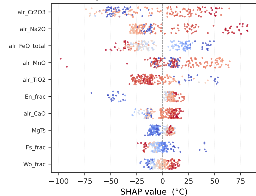
(c) Opx only · T (°C) shown: LightGBM/alr (TabPFN winner has no SHAP)
