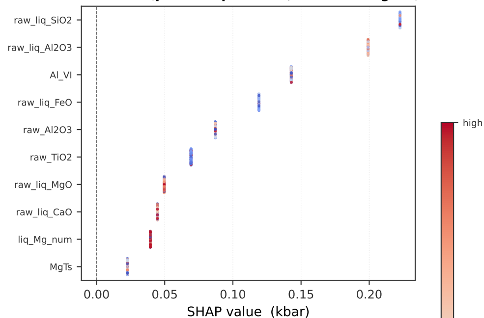
(b) Opx + Liquid · P (kbar) MLP/raw (perm. importance, SHAP surrogate)
