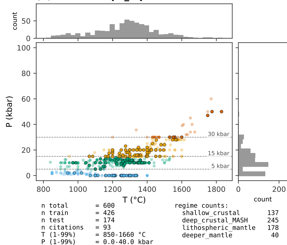
(a) ExPetDB opx_liq n=600
