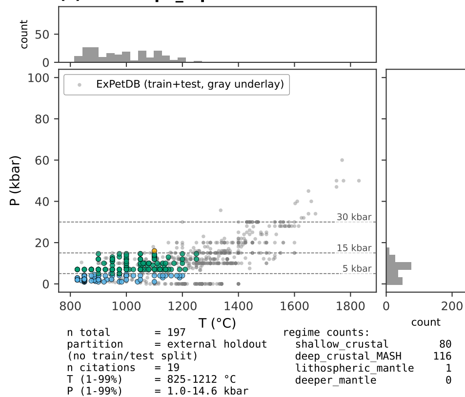
(c) ArcPL opx_liq held-out n=197
