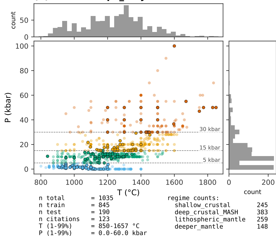
(b) ExPetDB opx_only n=1035
