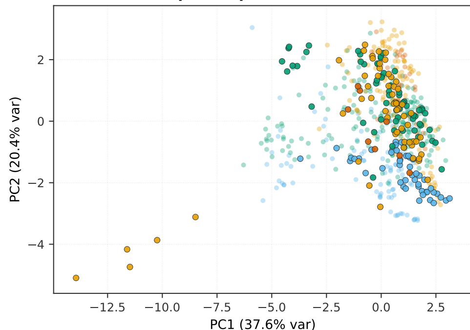
(a) ExPetDB · Opx + Liquid
