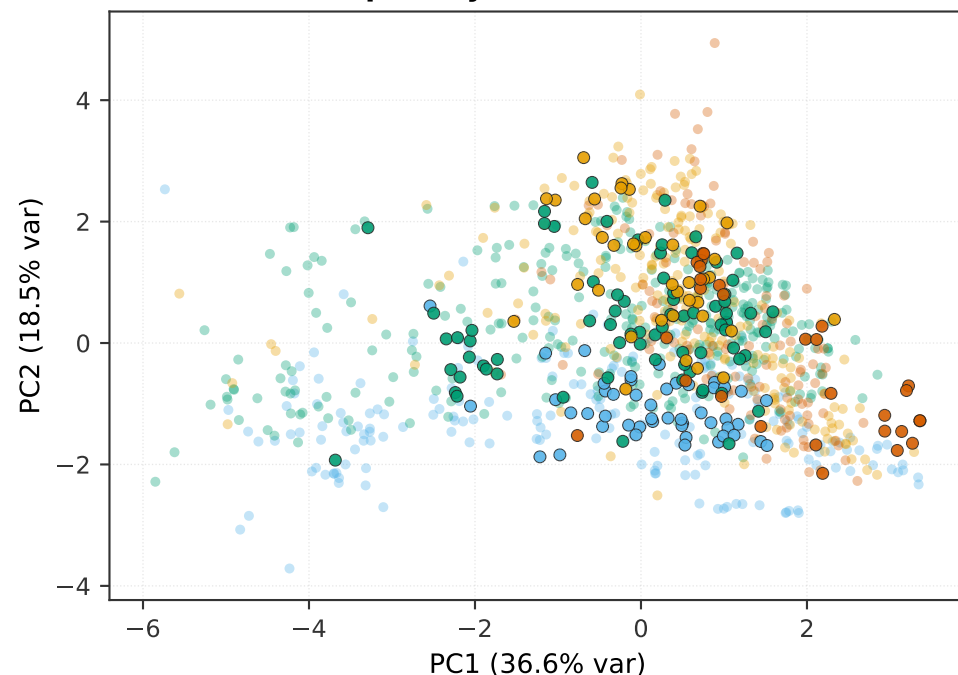
(b) ExPetDB · Opx only
