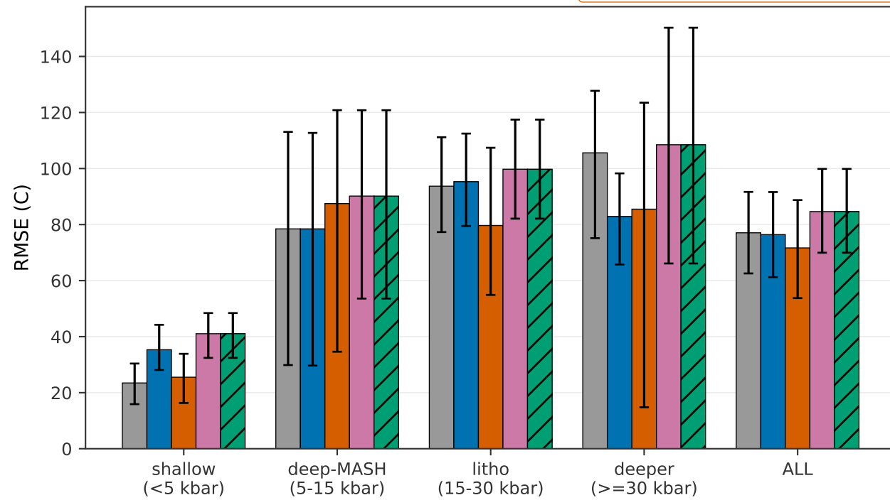
(a) Opx + Liquid T (C)
