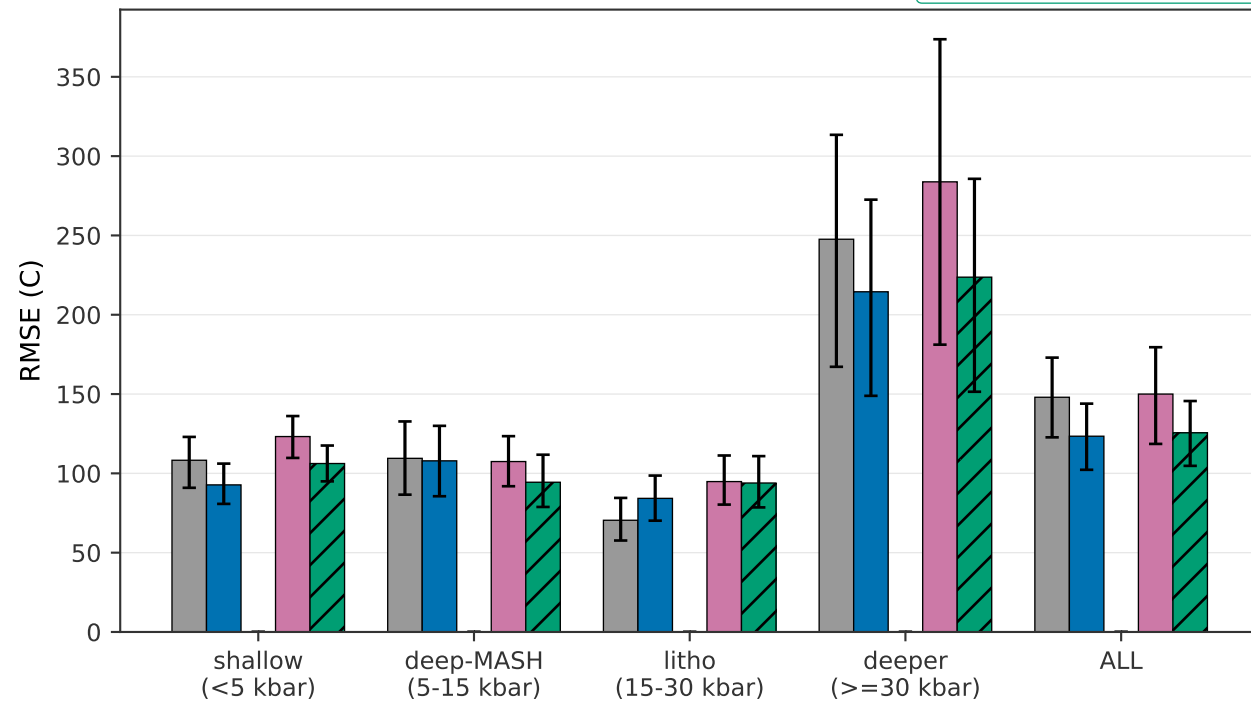
(c) Opx only T (C)
