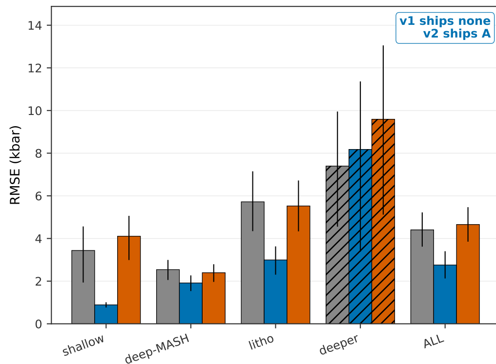
(b) Opx + Liquid P (kbar) corrected model: MLP + raw
