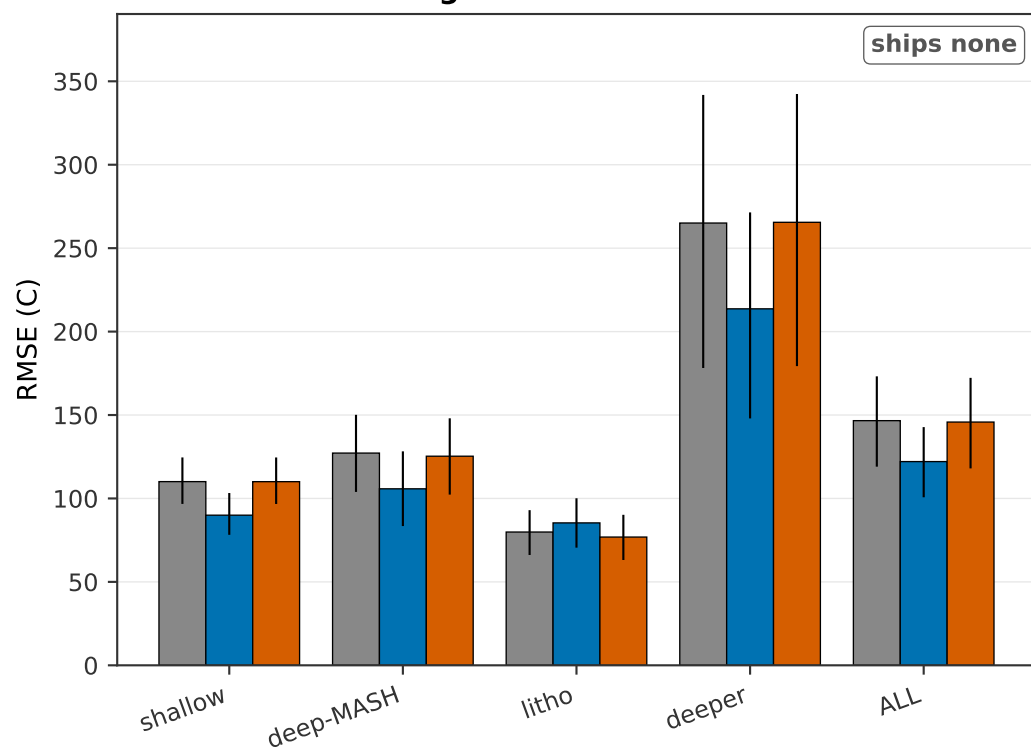
(c) Opx only T (C) corrected model: LightGBM + alr
