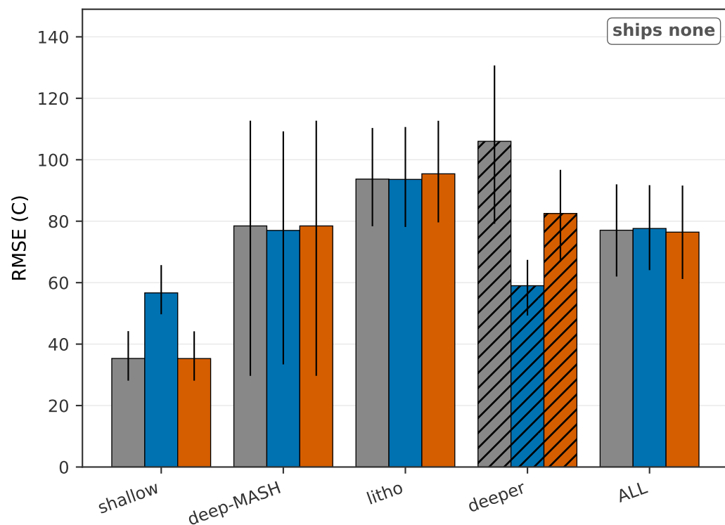
(a) Opx + Liquid T (C) corrected model: ElasticNet + raw
