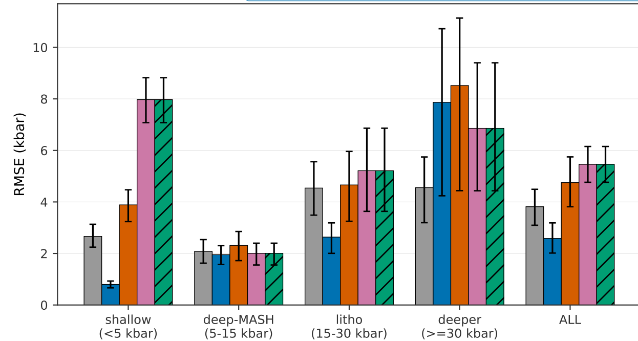
(b) Opx + Liquid P (kbar) ALL lowest RMSE (diagnostic): v10_corrected [MLP/raw]
