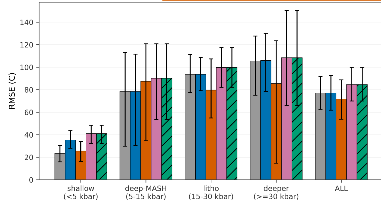
(a) Opx + Liquid T (C) ALL lowest RMSE (diagnostic): external [Putirka 28a]
