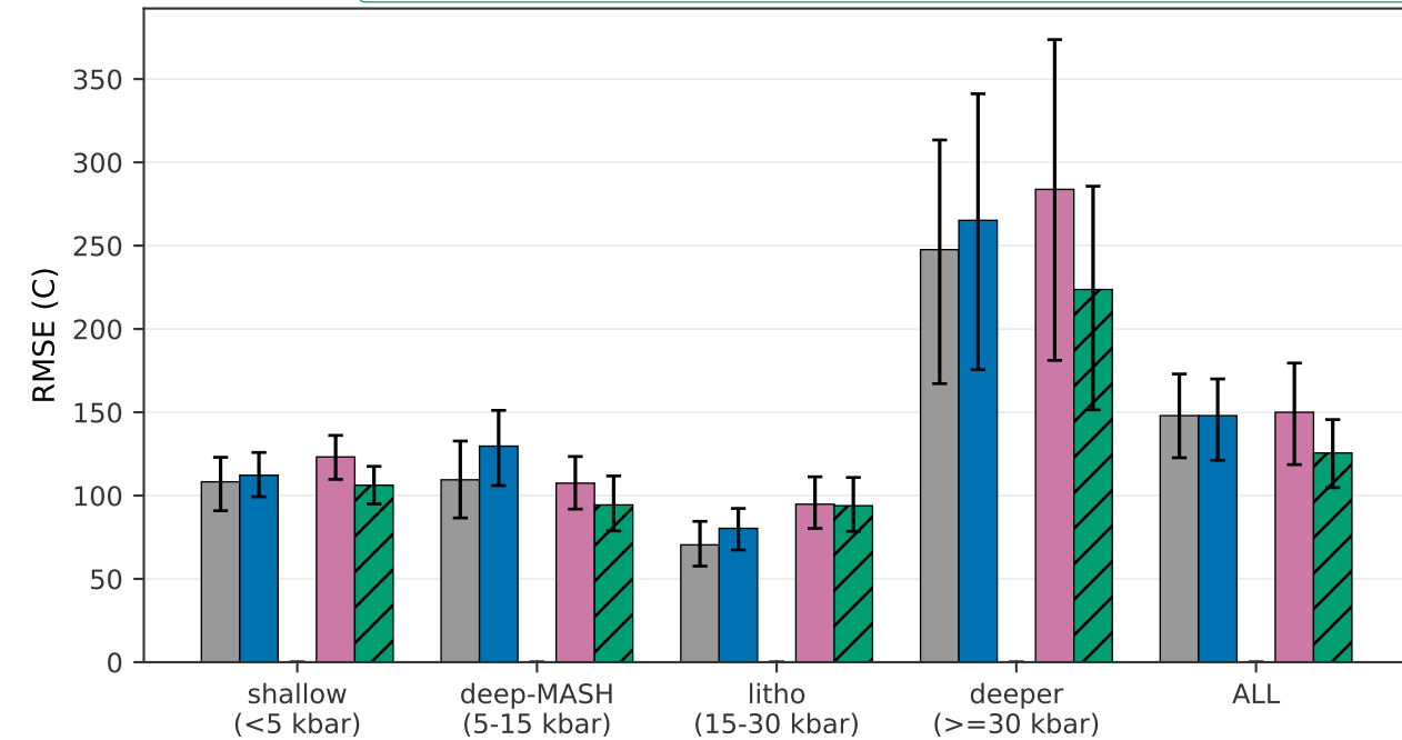
(c) Opx only T (C) ALL lowest RMSE (diagnostic): tabpfn_corrected [TabPFN/raw (post)]
