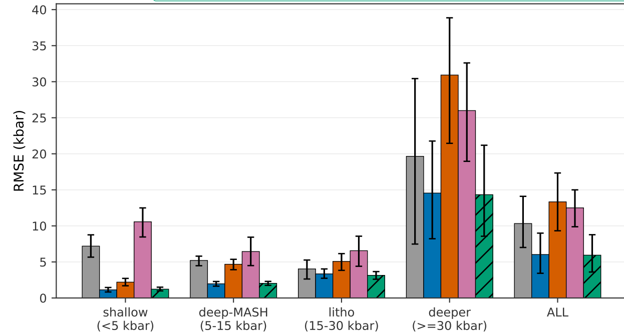
(d) Opx only P (kbar) ALL lowest RMSE (diagnostic): tabpfn_corrected [TabPFN/raw (post)]
