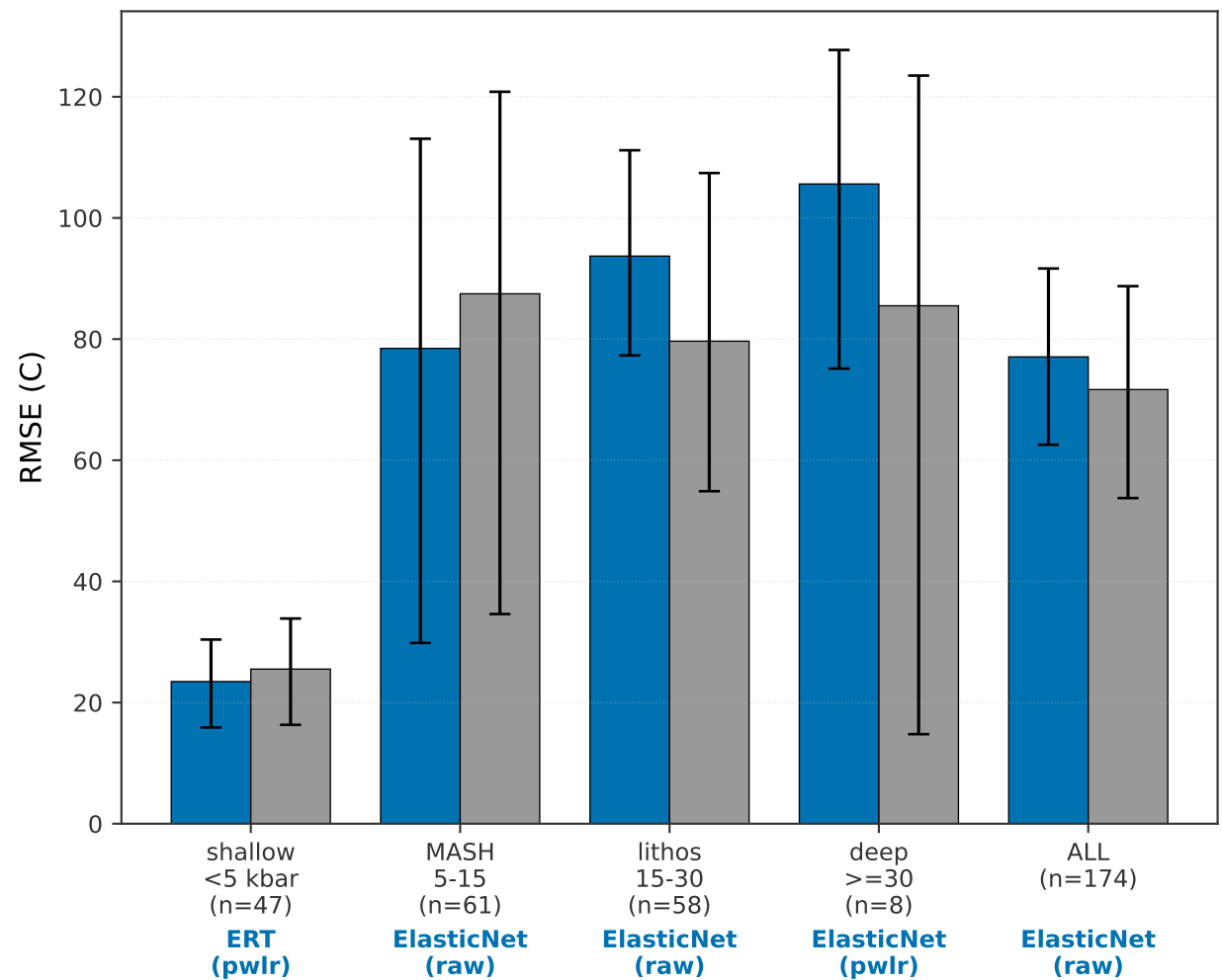
(a) Opx + Liquid T (C)
