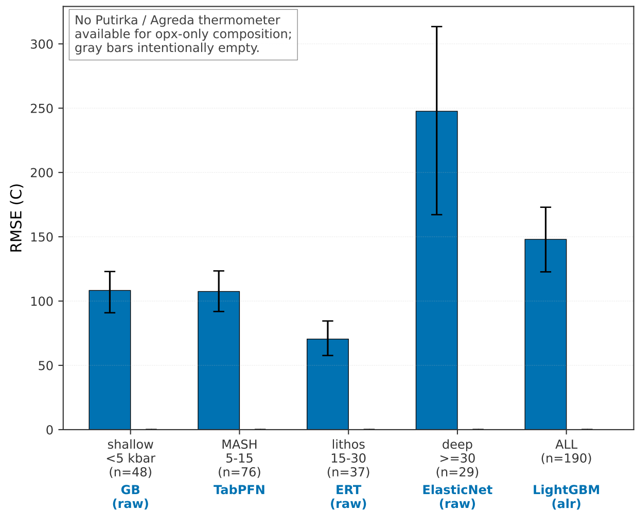
(c) Opx only T (C)
