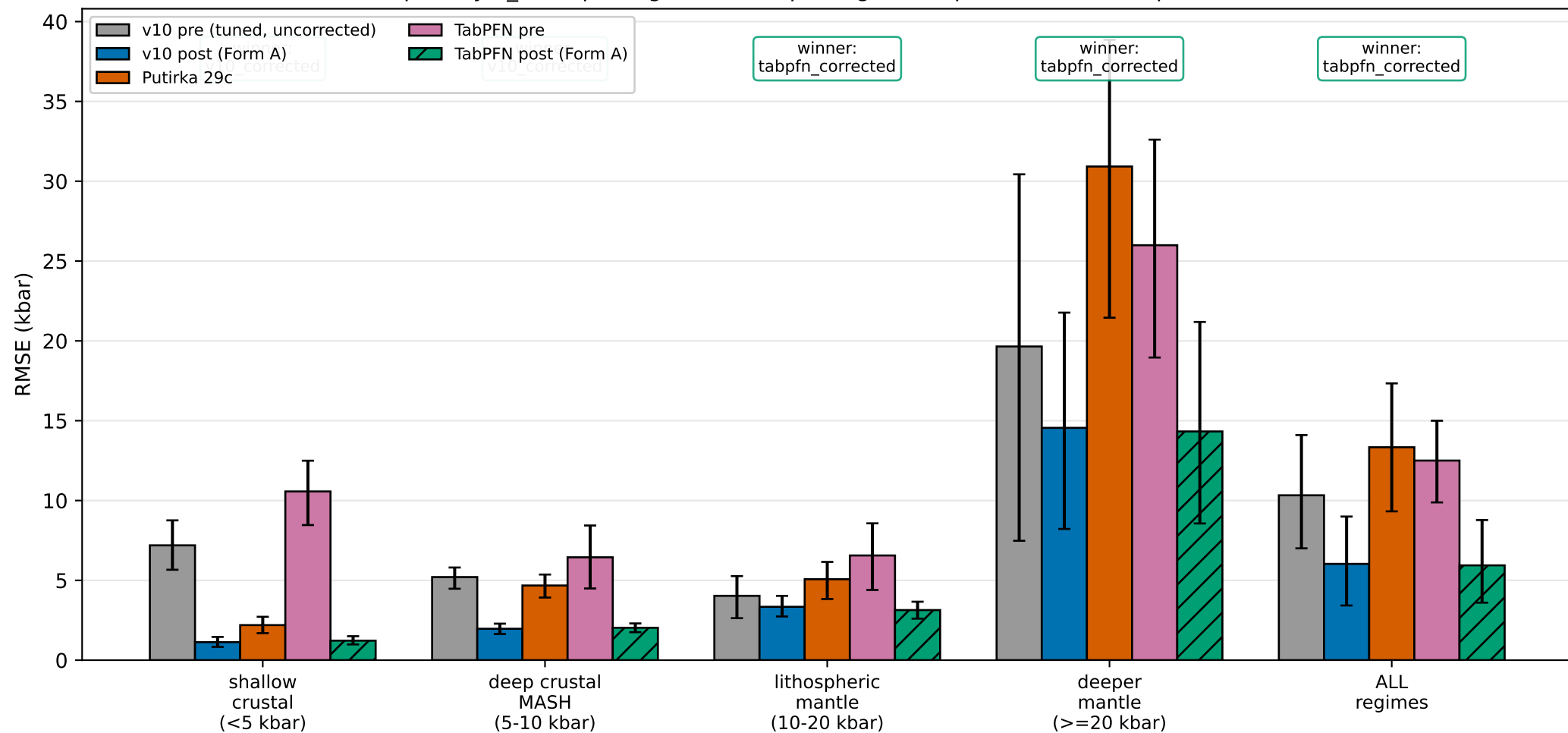
opx-only P_kbar: per-regime RMSE (pre-registered partition, bootstrap 95% CI)
