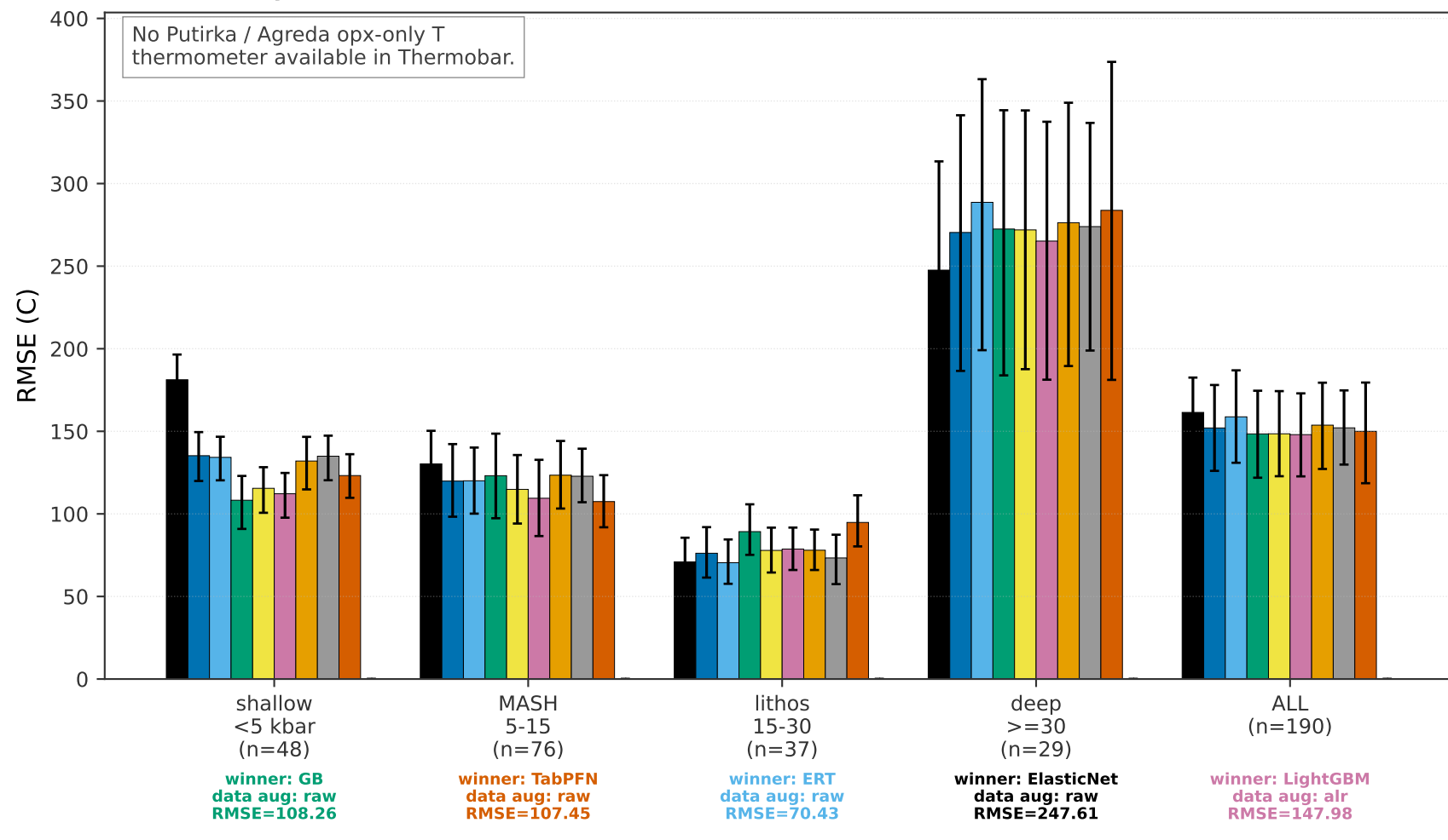
(c) Opx only T (C)
