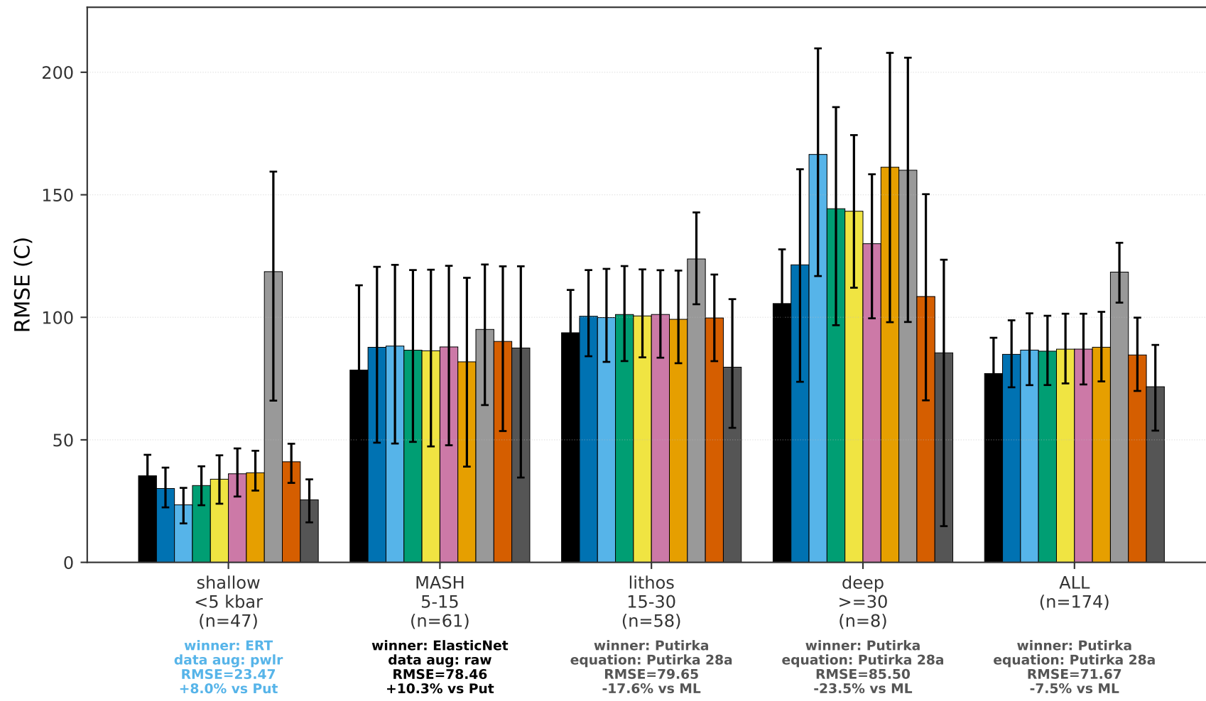
(a) Opx + Liquid T (C)
