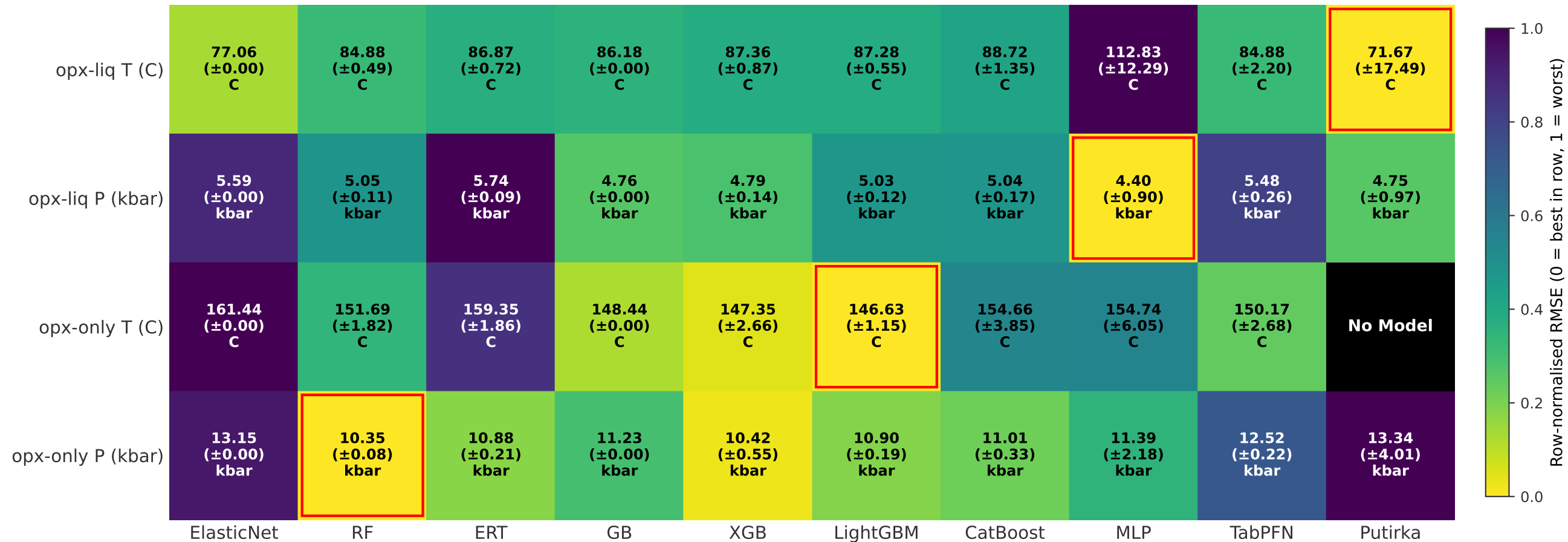
Overall test-set RMSE heatmap -- 4 opx combos x 10 candidates (cell text = mean RMSE \pm half-width of 95% CI; viridis colormap, row-normalised; thin red outline = best per row)
