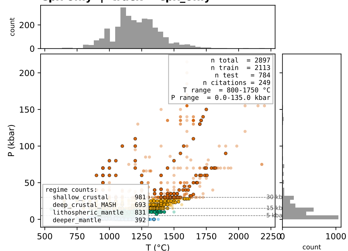
Cpx only | track = cpx_only
