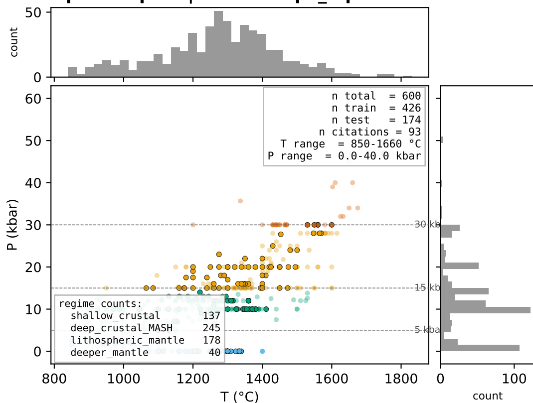
Opx + Liquid | track = opx_liq
