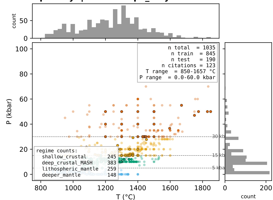
Opx only | track = opx_only
