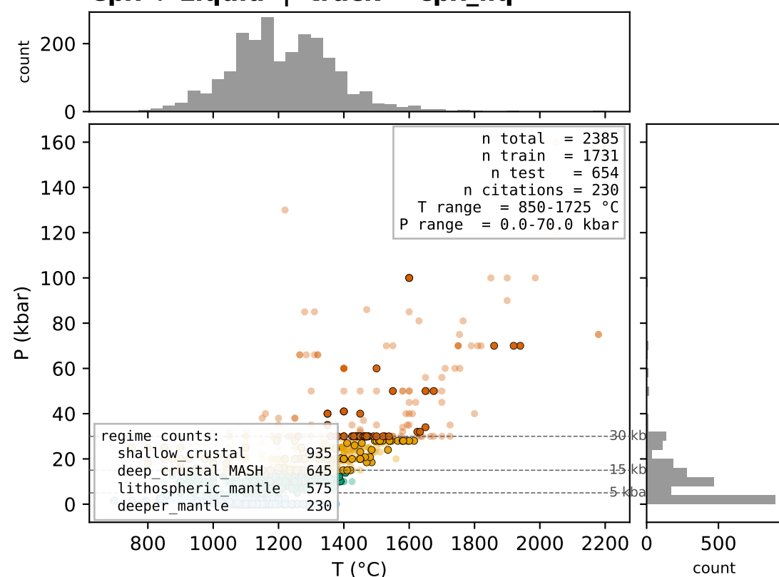
Cpx + Liquid | track = cpx_liq
