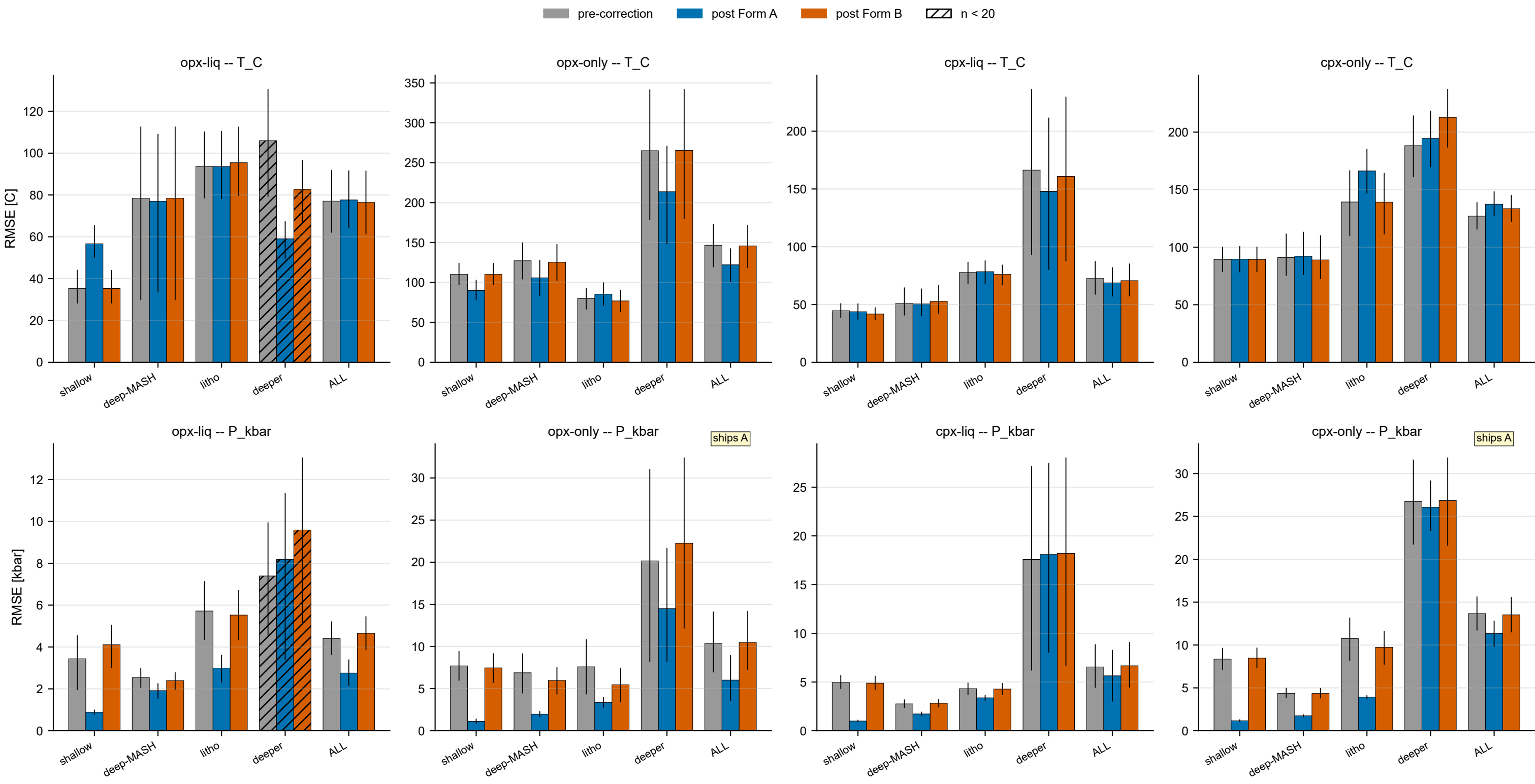
Figure 30. Per-regime test-set RMSE (20-seed mean with bootstrap CI envelope)
