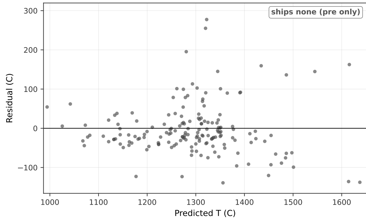
(c) Opx only T (C) corrected model: LightGBM + alr
