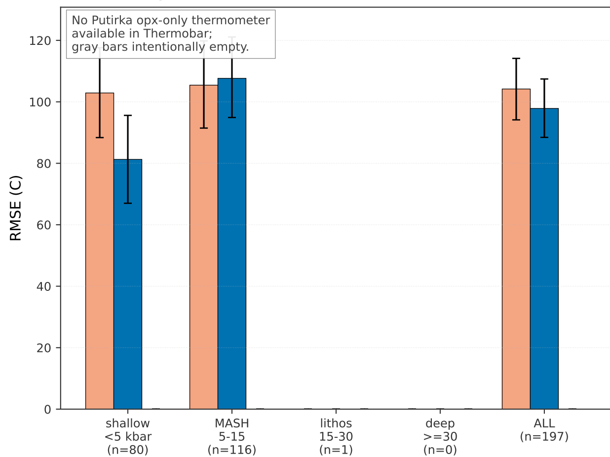
(c) Opx only T (C)
