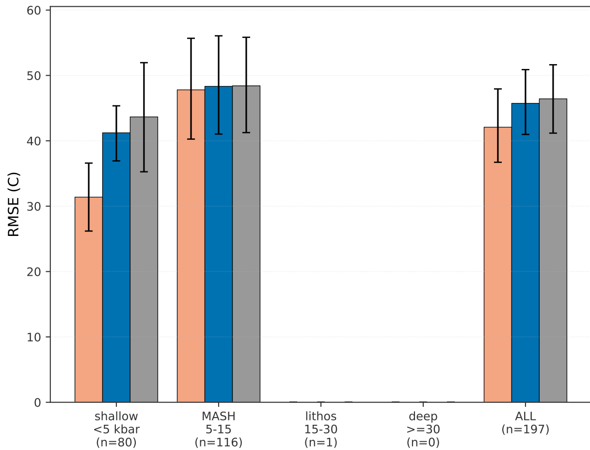
(a) Opx + Liquid T (C)
