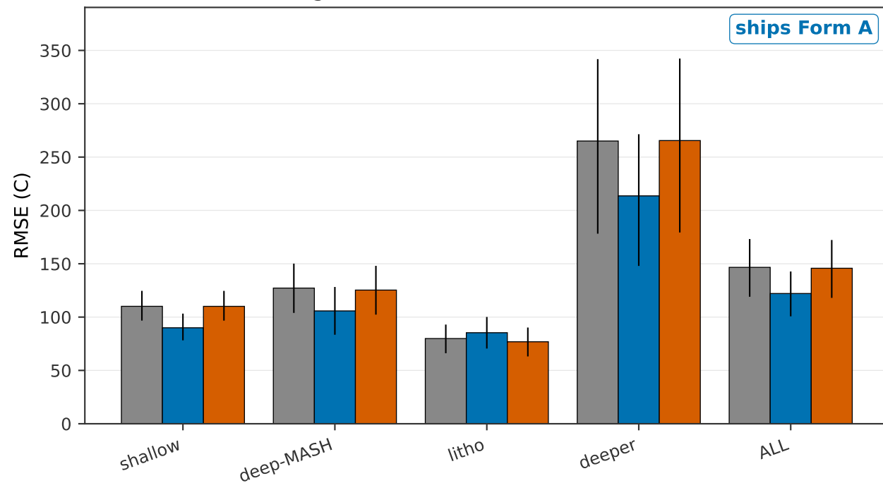
(c) Opx only T (C) corrected model: LightGBM + alr
