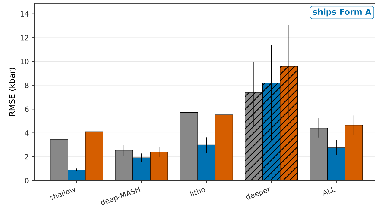
(b) Opx + Liquid P (kbar) corrected model: MLP + raw
