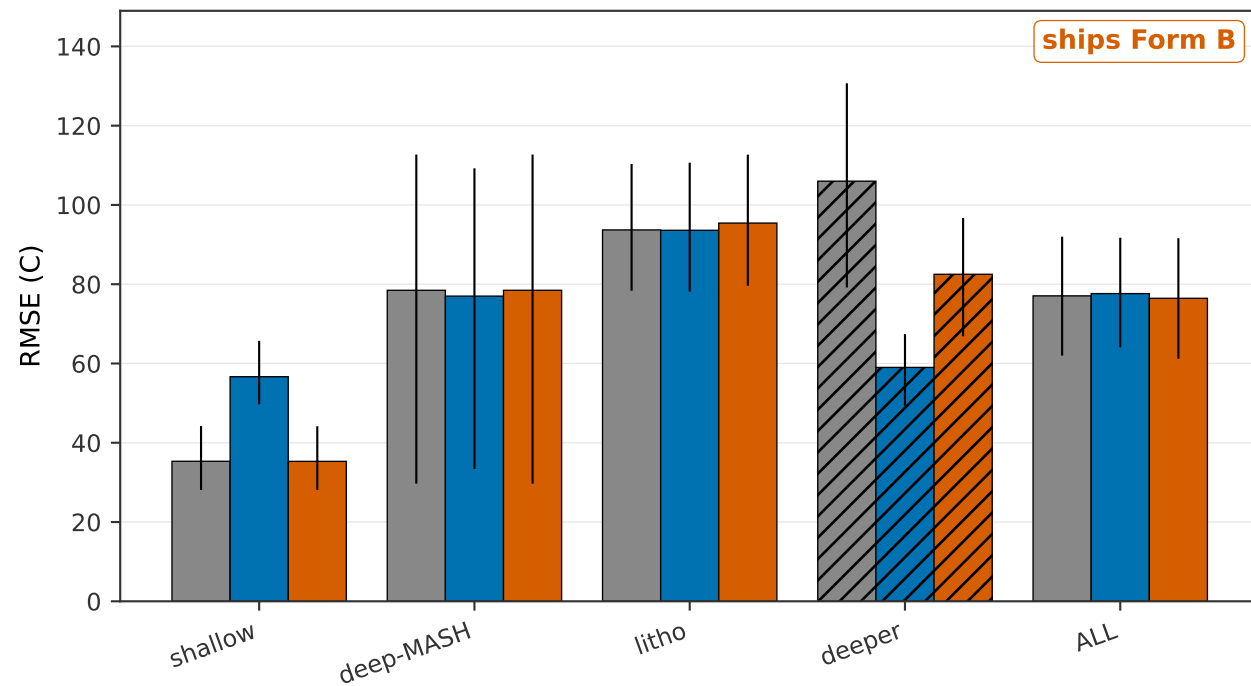
(a) Opx + Liquid T (C) corrected model: ElasticNet + raw
