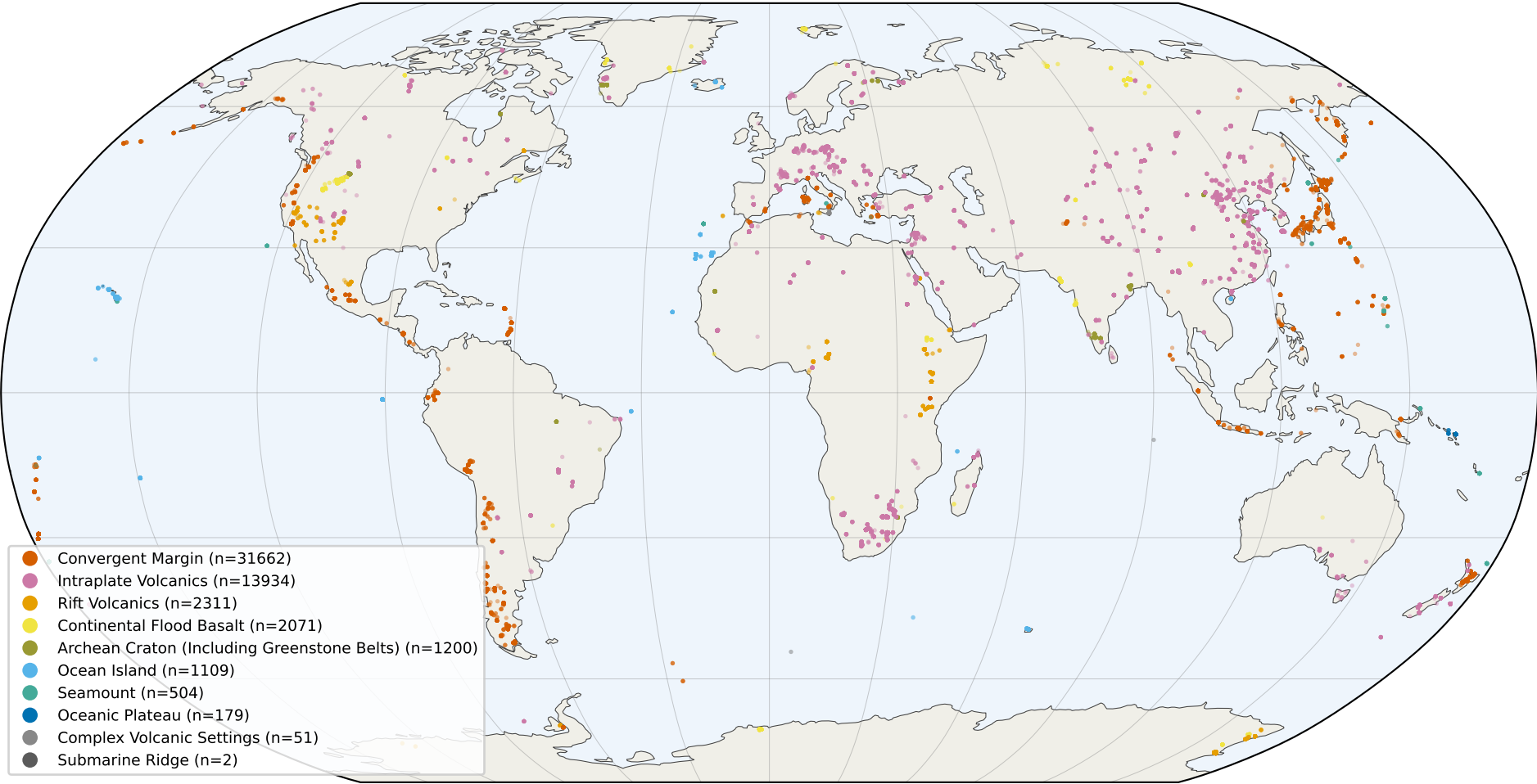
A. OPX natural samples by tectonic setting (n=53023)
