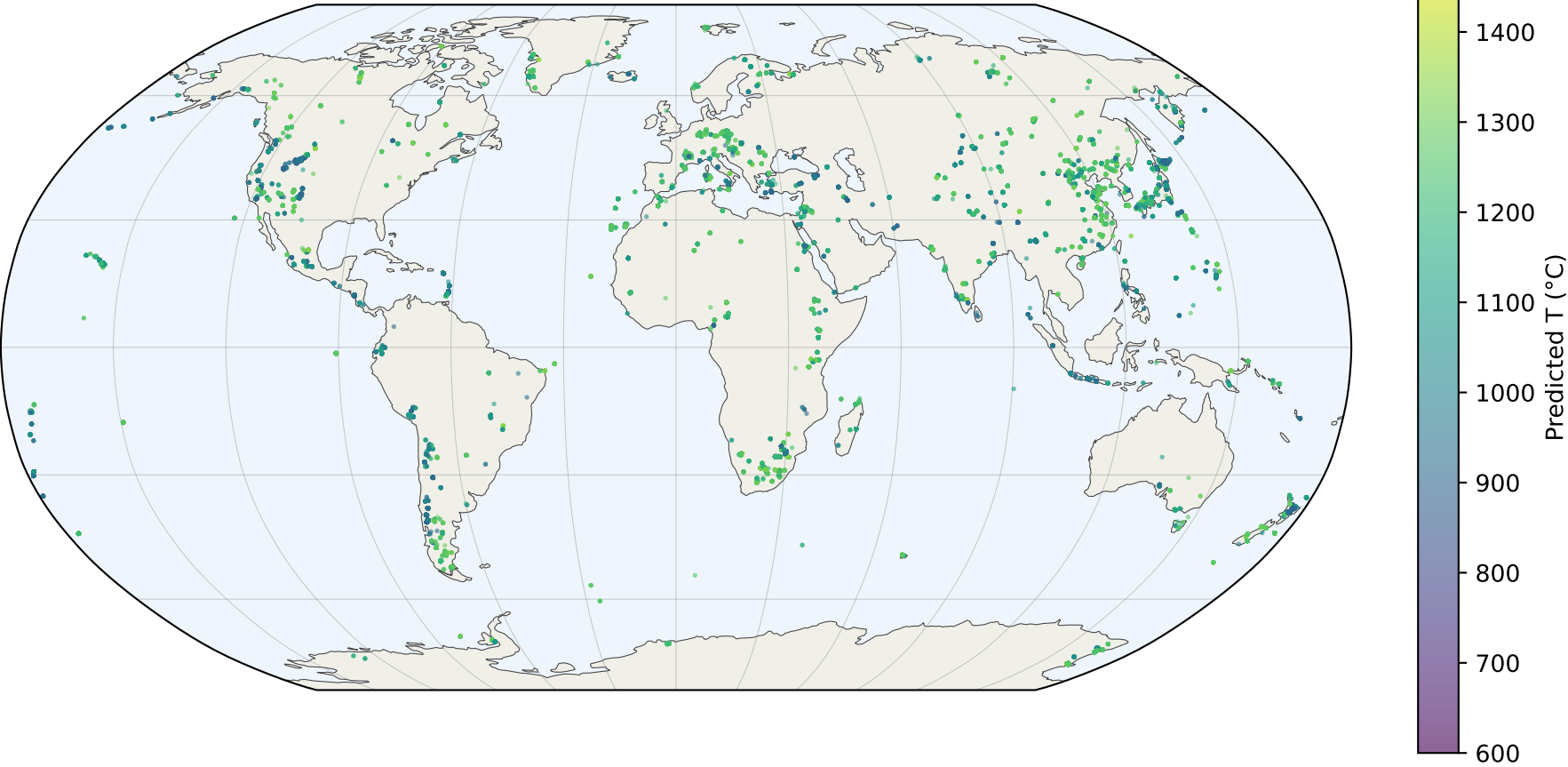
B. OPX predicted T (canonical model, n=53023)
