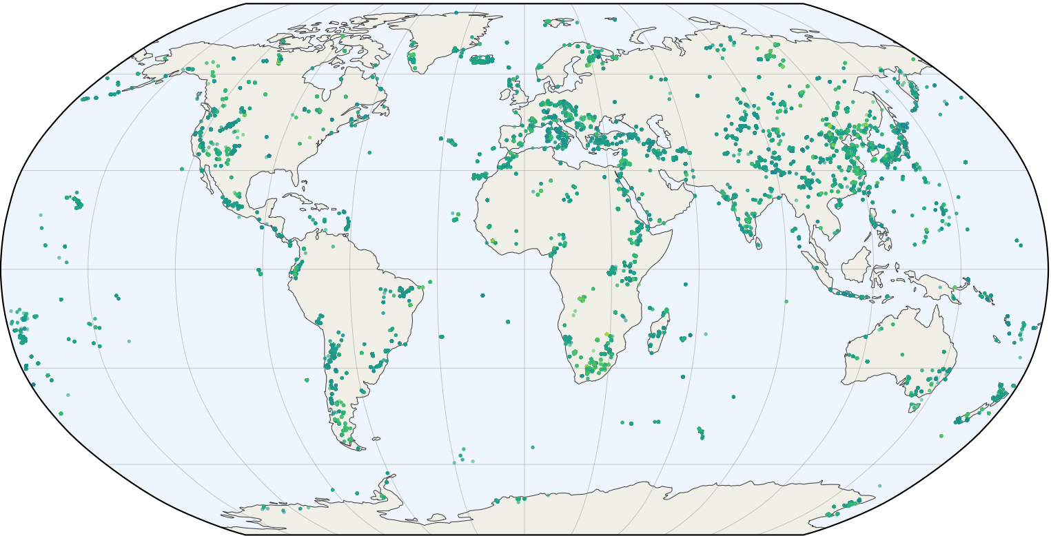
B. CPX predicted T (canonical model, n=93125)
