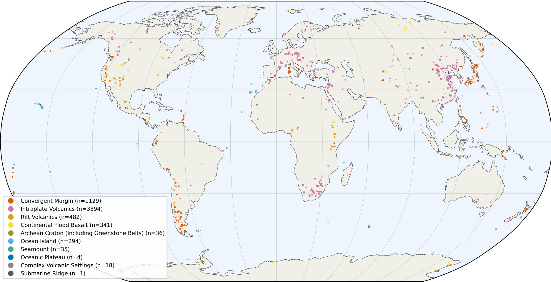
A. TWOPX natural samples by tectonic setting (n=6234)
