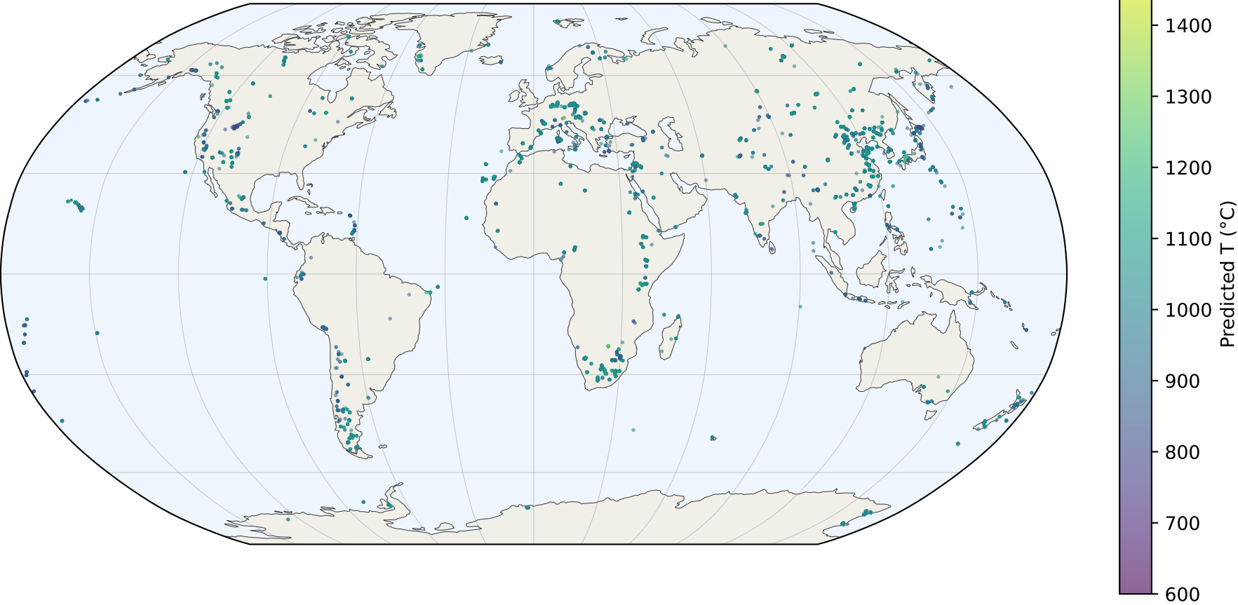
B. TWOPX predicted T (canonical model, n=6234)
